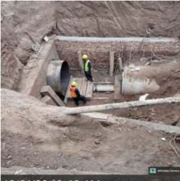
Picture 72: Pipe Laying through Thrust Boring in Process
